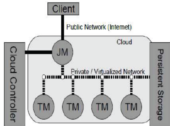
Fig. 3 Design Architecture of Nephelē Framework [4]
