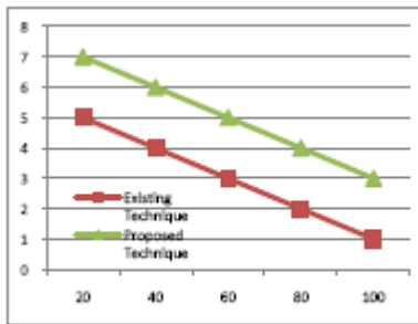
Fig. 4. Route reliability.
