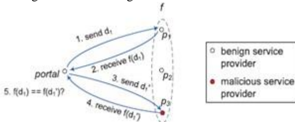
Figure 3: Consistency check
