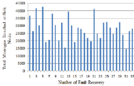
Fig. 16. Total messages reaching the sink node for each replaced node.
