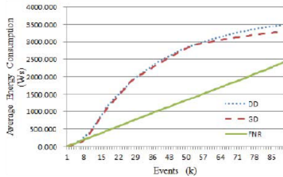
Fig. 10. Average energy consumption.
