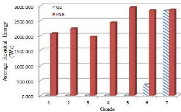
Fig. 14. Average residual energy after 90000 events.
