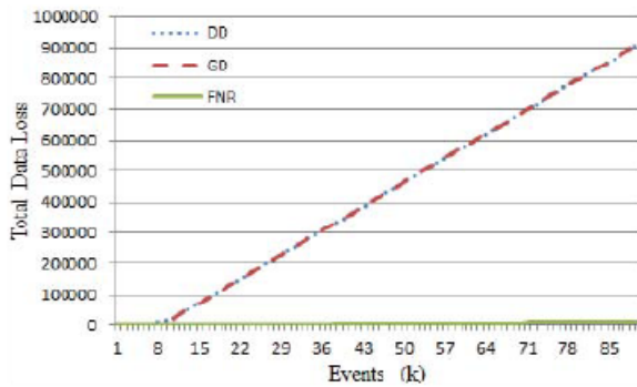
Fig. 9. Total data loss.
