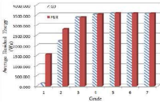
Fig. 13. Average residual energy after 8000 events.
