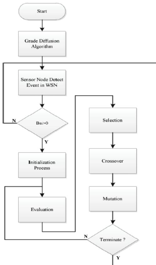
Fig. 3. Fault node recovery algorithm flow chart.
