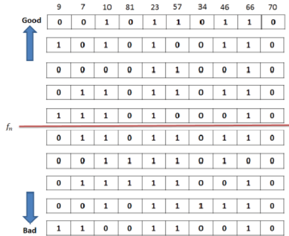
Fig. 5. Selection step.
