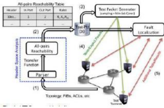
Fig. 4. ATPG system block diagram.
