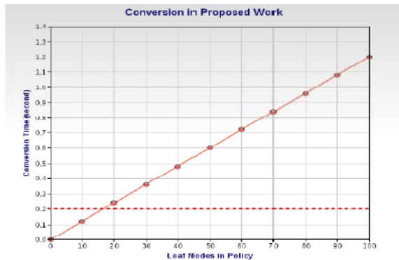
Fig. 4. d) Conversion in Proposed works
