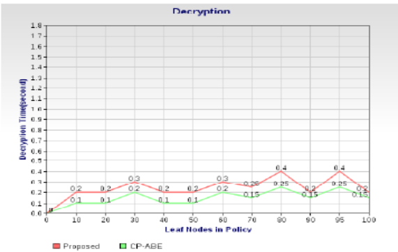
Fig. 4. c) Decryption
