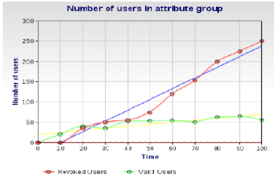
Fig. 4. b) the number of users in an attribute groups
