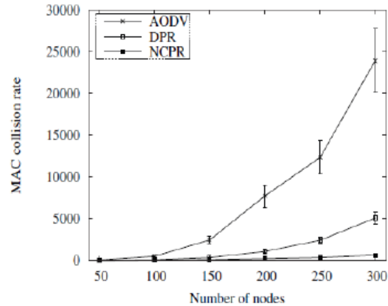
Fig 1. Collision rate with varied number of nodes
