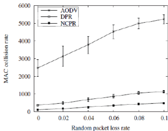
Fig 3. Collision rate with varied random packet loss rate
