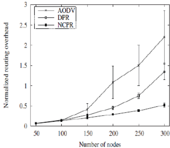
Fig 2. Normalized routing overhead with varied number of nodes
